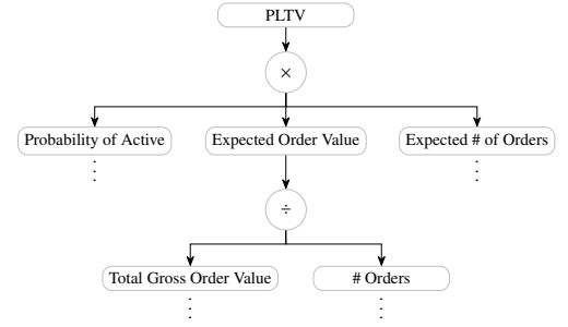
Figure 1: (Left) Transformations for computing Predicted Life-Time Value (PLTV), where Prob Active, Expected # Orders denote probability of active, and expected number of orders, respectively. (Right) Example PLTV submetric hierarchy decomposition.
